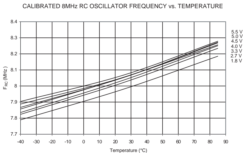
Figure 131. Calibrated 8 MHz RC Oscillator Frequency vs. Temperature
