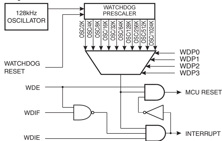
Figure 20. Watchdog Timer
